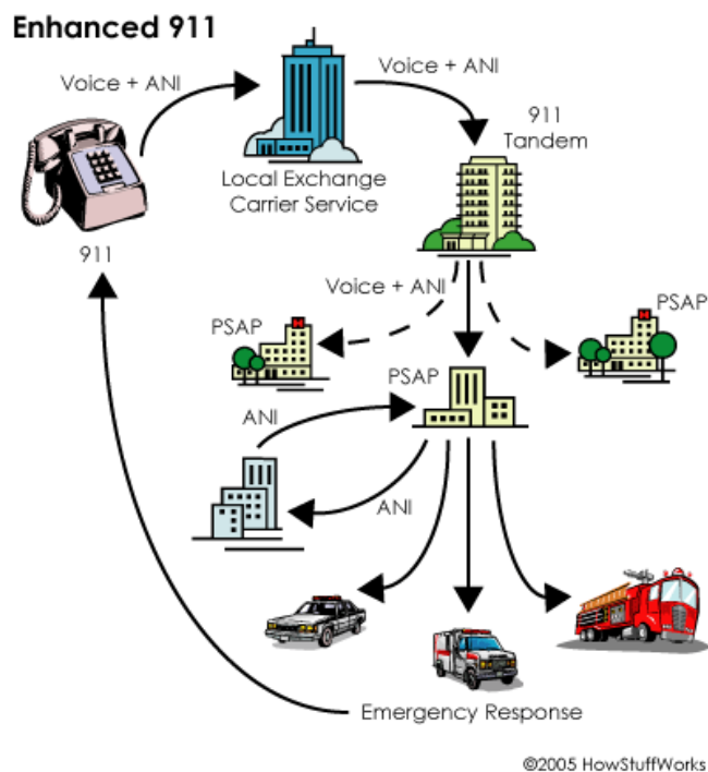
Obr. 23 Systém E911 [75]
